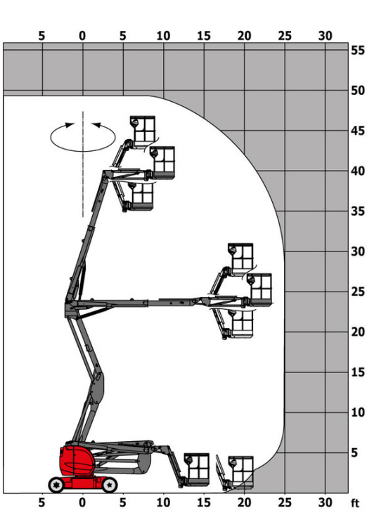
Load Chart imperial
