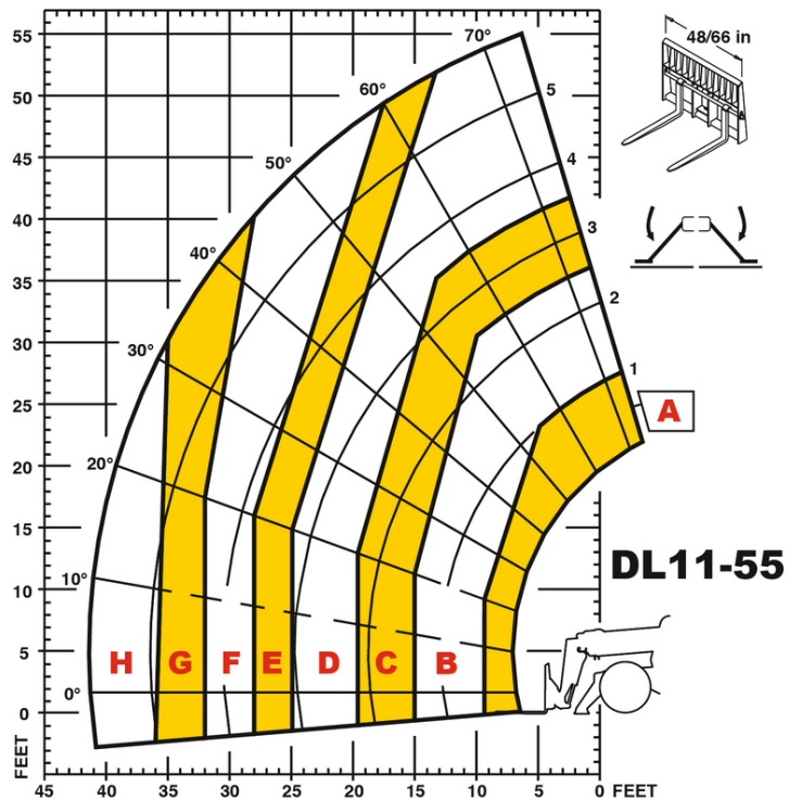
Machine on stabilizers with forks Imperial
