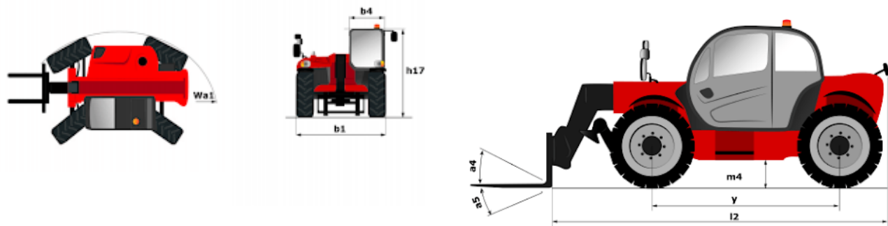
MTA 12042 Series IV - Dimensional drawing
