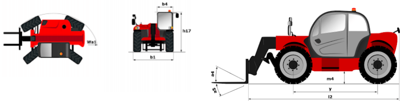
MTA 10055 E74 - Dimensional drawing
