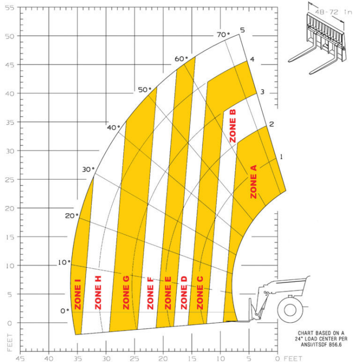
Load Chart imperial
