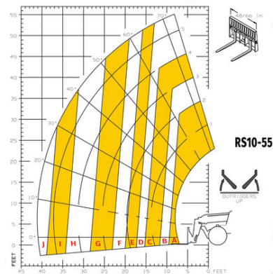
Load Chart imperial
