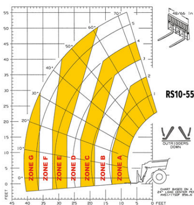
Machine on stabilizers with forks Imperial
