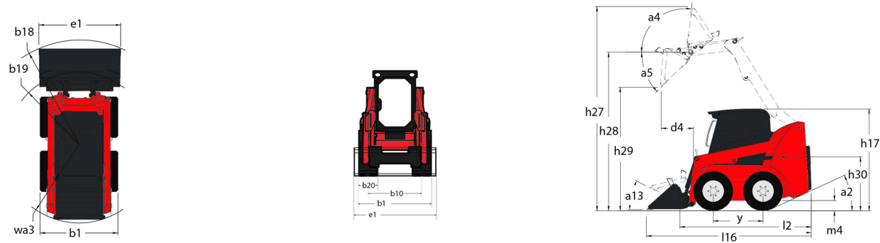
2600R - Dimensional drawing
